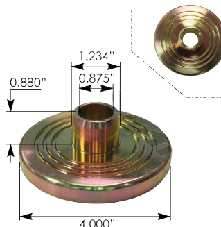
Concentric Collar Hendrickson PN: MHS97
