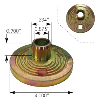
Eccentric Collar Hendrickson WWPN: MHS99
