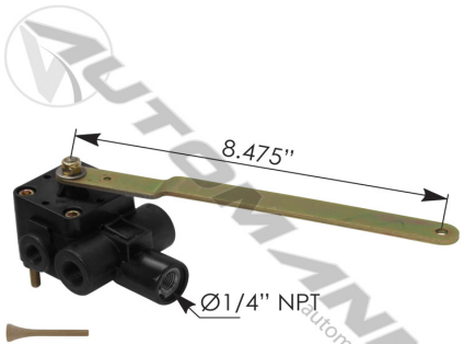
Hendrickson Height Control Valve PN: 171.501OE
